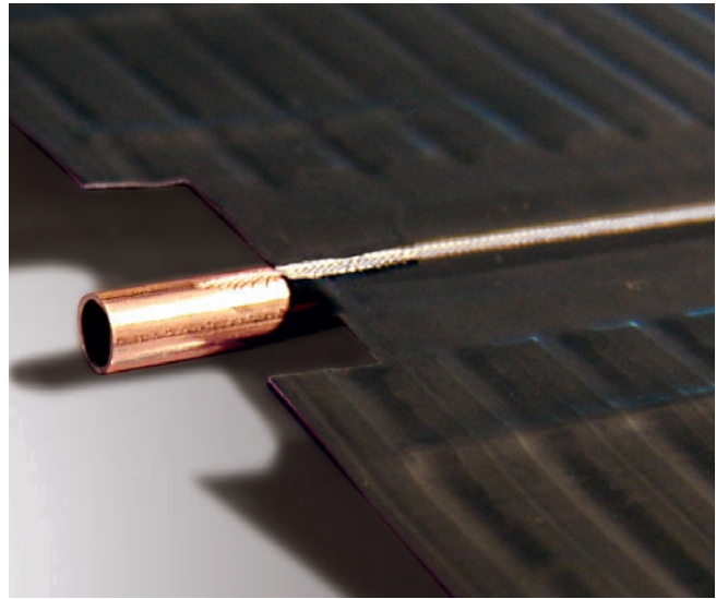
solarclean® copper tubes for efficient solar heat absorbers with a long life expectancy
